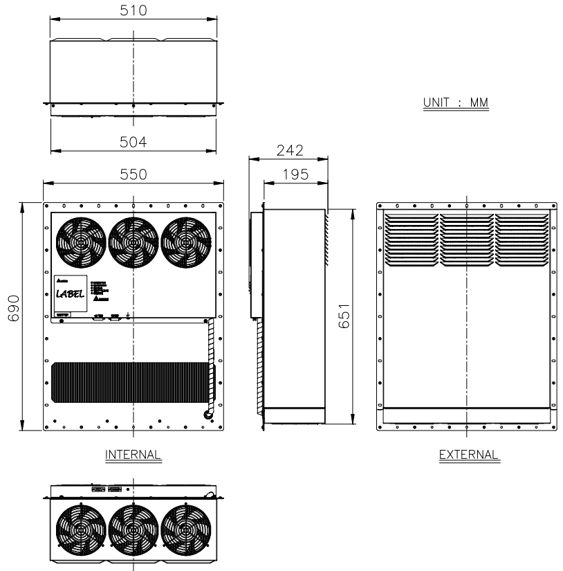
Dimension drawing
