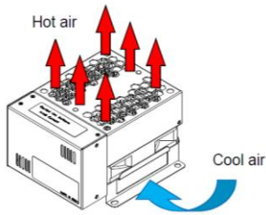
Airflow orientation
