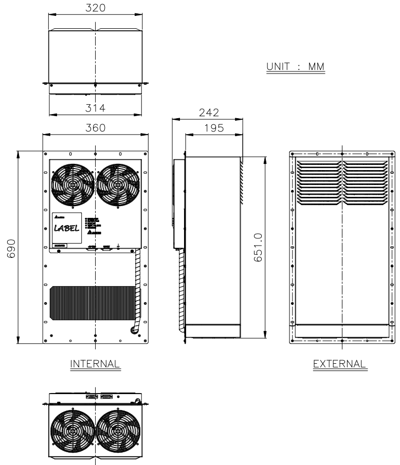
Dimension drawing
